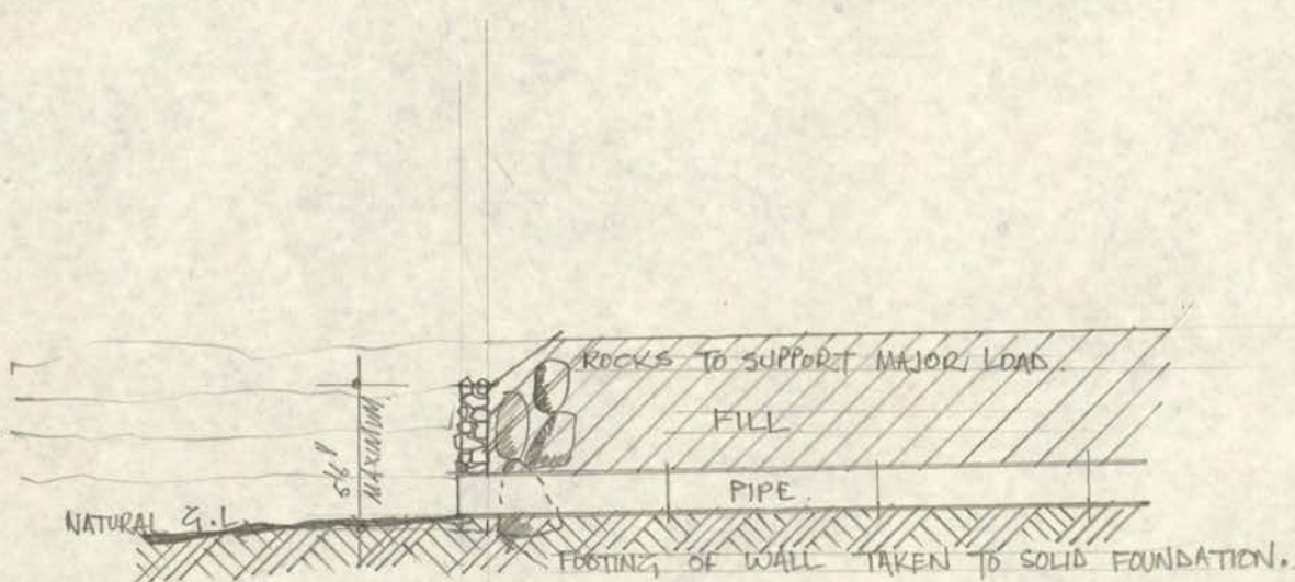
SECTION OF TYPICAL HEADWALL.
